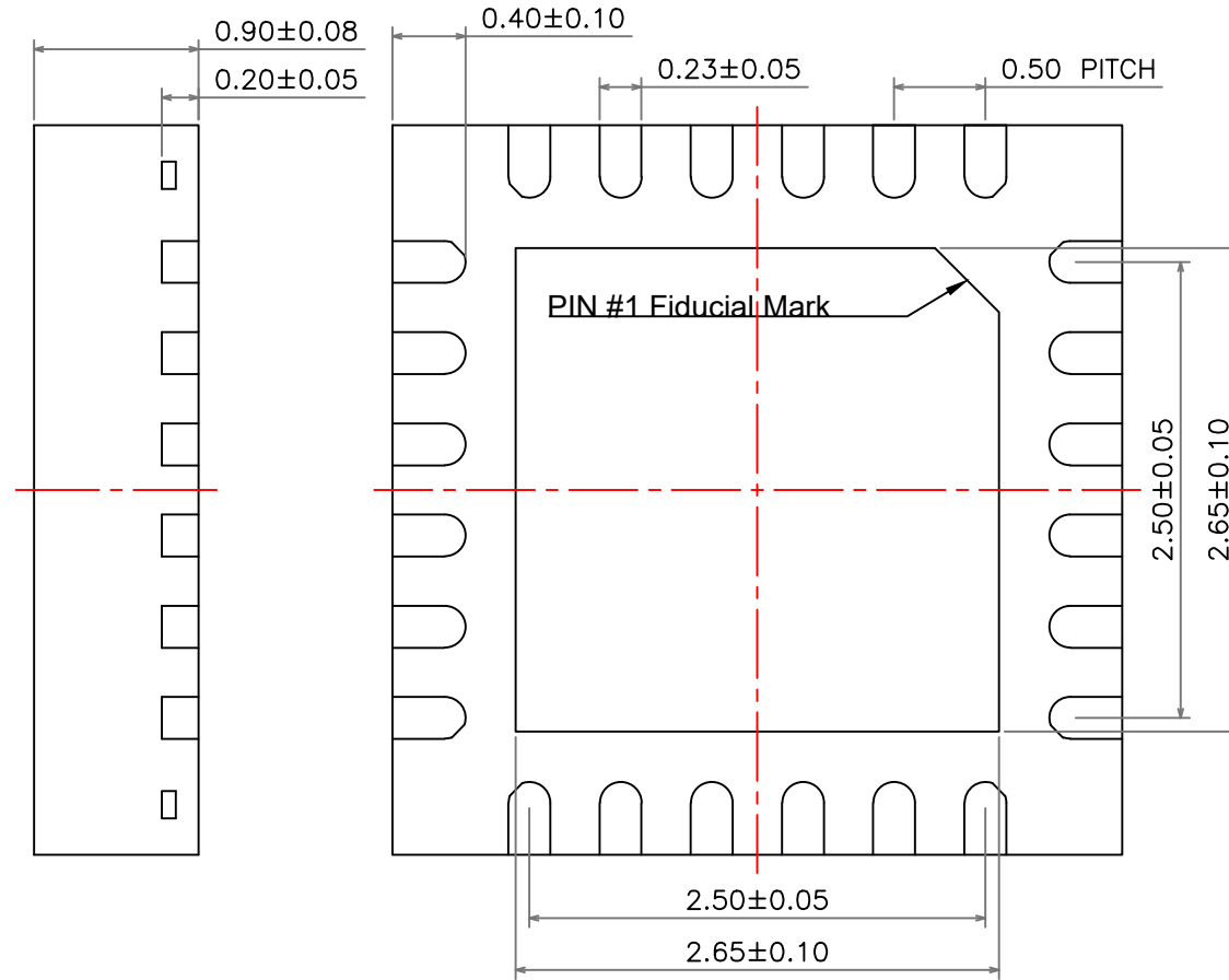
SIDE VIEW
